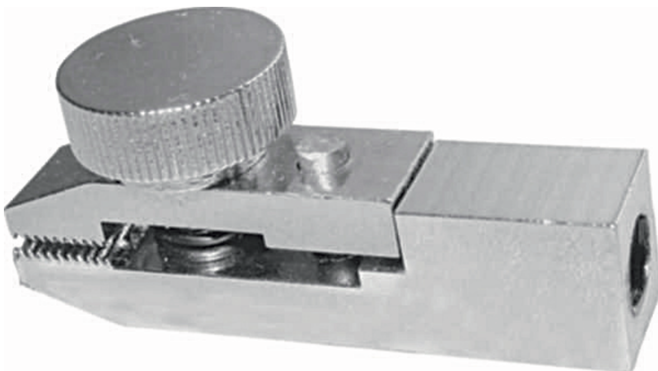
Long clamp for tension and rupture tests
